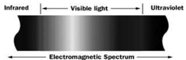
Fig2: spectrum of light
